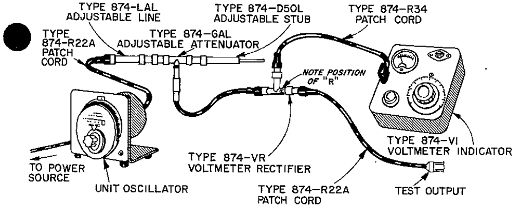
Figure 5. Block diagram of a simple signal generator using the adjustable attenuator and other Type 874 Coaxial Elements.
