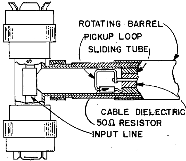
Figure 1. Cutaway view of adjustable attenuator.
