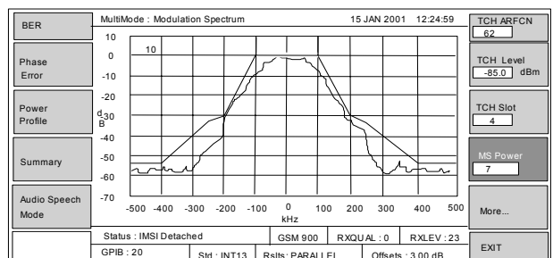
Real time displays for simple adjustments with superimposed limit mask
